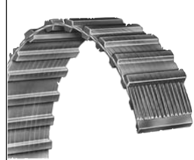
Synchro-Link® Double Sided Timing Belts (XL, L, H Rubber) (MXL, XL, T5, T10 Polyurethane) Designed for synchronized serpentine drives, these belts position teeth on both sides of the belt to provide smooth, precise performance under exacting drive conditions.
